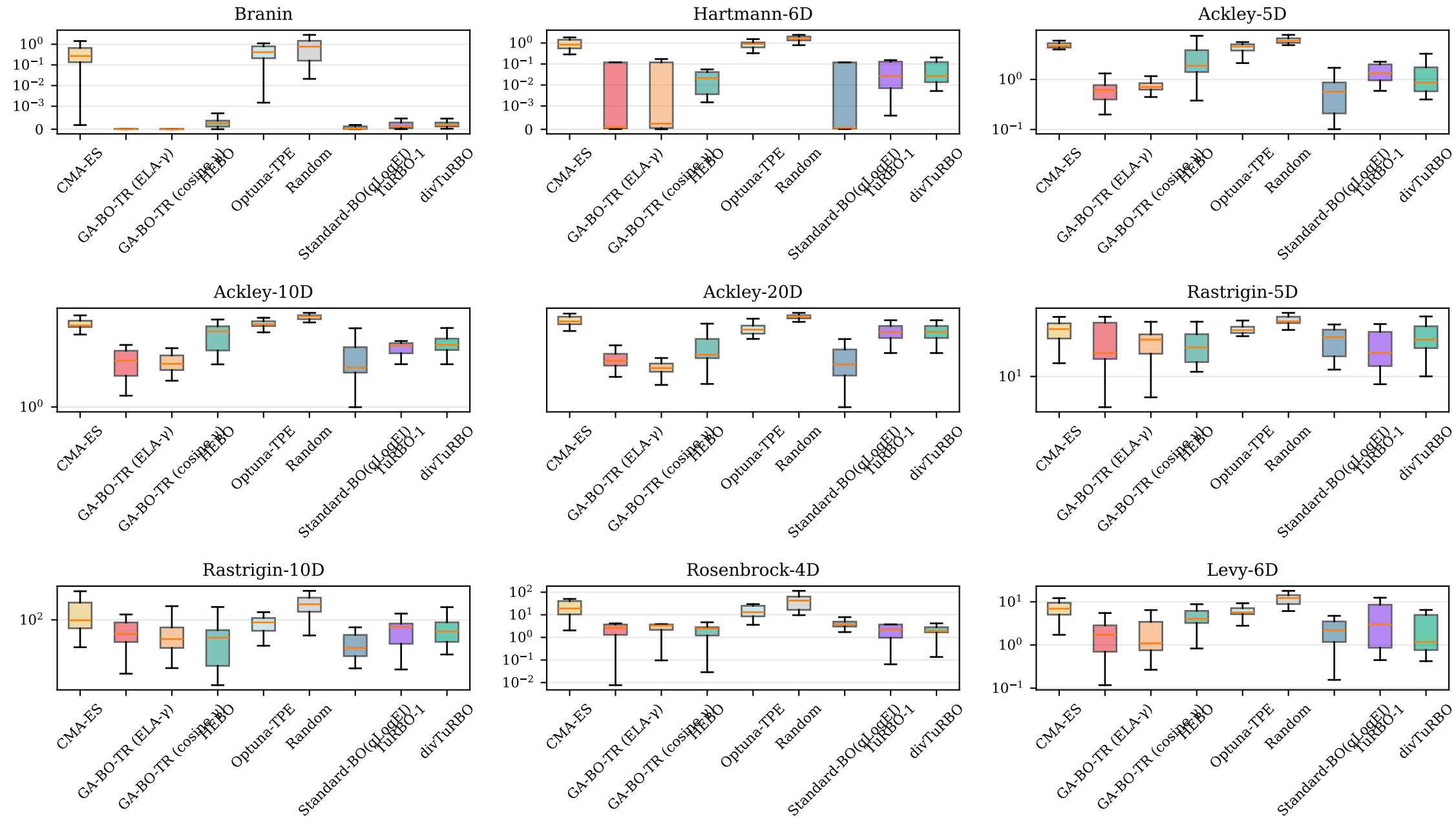
Final regret distribution (lower is better)
